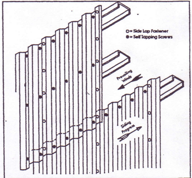
TYPICAL FASTENER LOCATIONS
