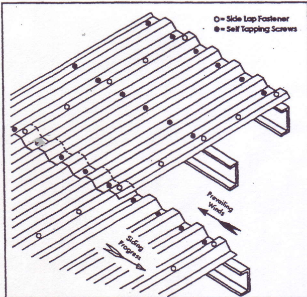
TYPICAL FASTENER LOCATIONS ROOFING
